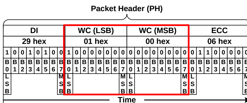
Figure 56 Word Count (WC) on the Long Packet (LPa)
